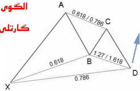
Bullish gartley
