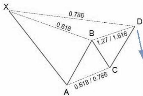
Bearish Gartley
